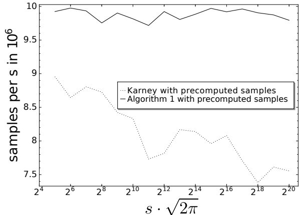
Figure 3: Performance of Algorithm 1 compared to Karney's algorithm, (online phase only).
