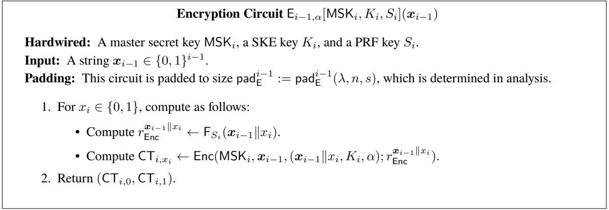
Figure 9: The description of \text{E}_{i-1,\alpha} for every i \in \{3, \dots, n\} and \alpha \in \{0, 1\} .
