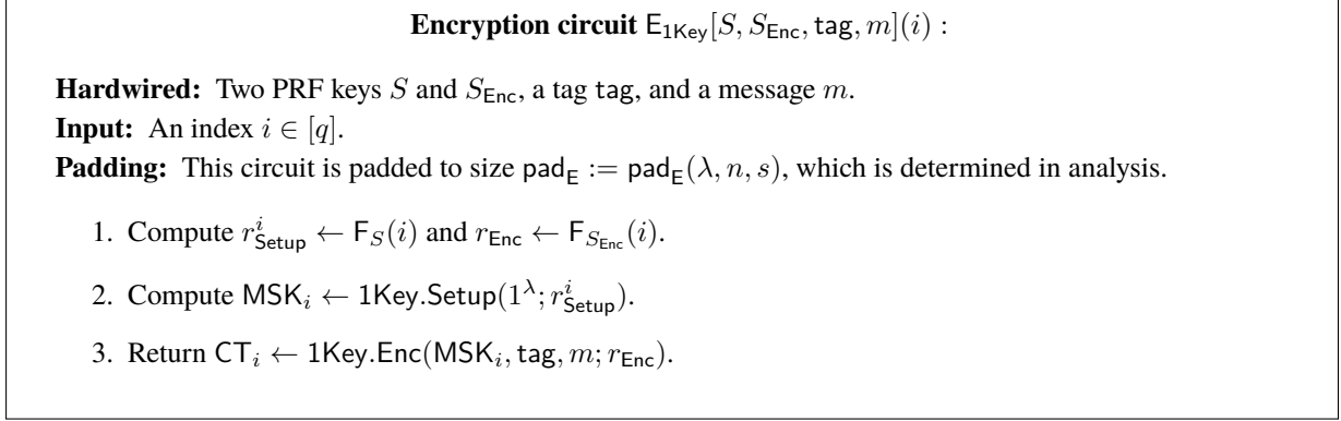
Figure 2: The description of E_{1\text{Key}} .
