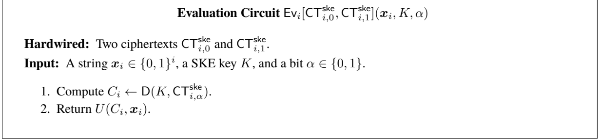
Figure 8: The description of \text{Ev}_i for every i \in \{2, \dots, n\} . In the description, U(\cdot, \cdot) is an universal circuit.
