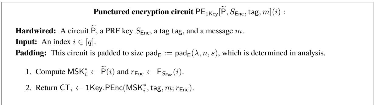
Figure 4: The description of \text{PE}_{1\text{Key}} .
