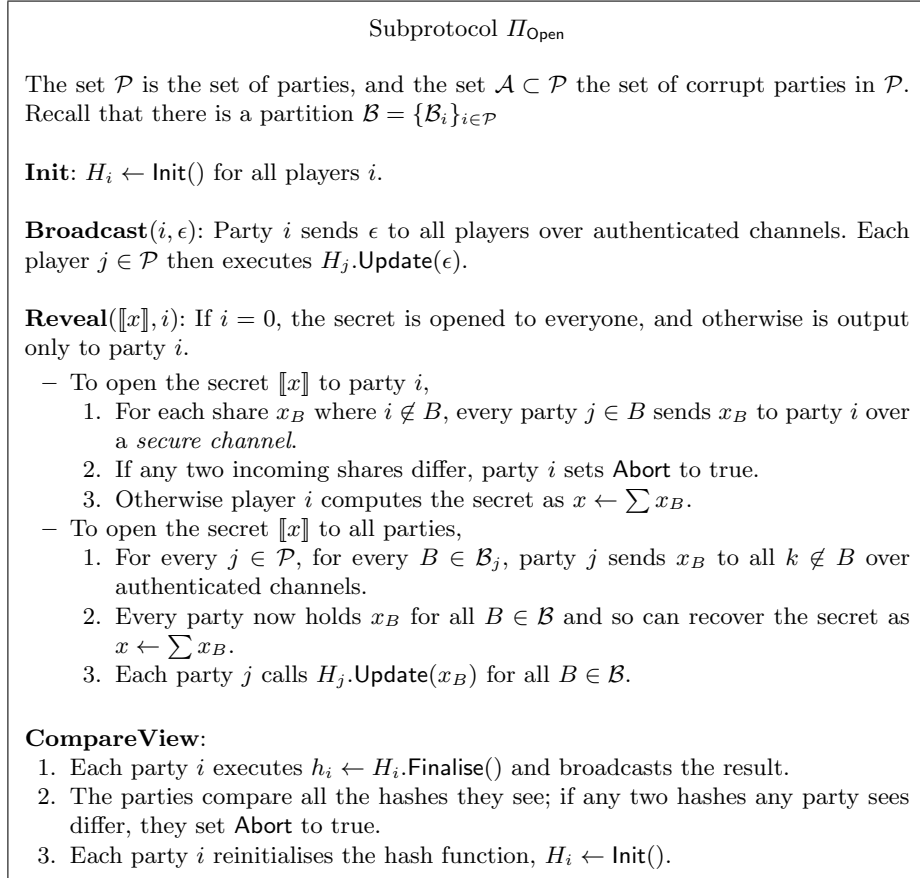
Figure 6. Subprotocol \Pi_{\text{Open}}
