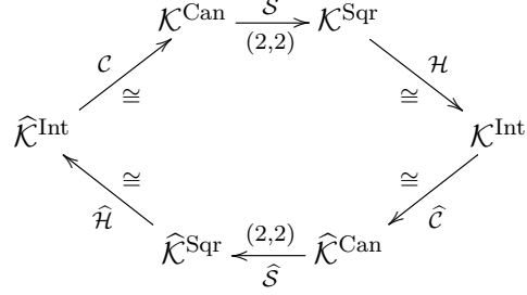
Fig. 1. Decomposition of pseudo-doubling on fast Kummer surfaces into a cycle of morphisms. Here, \mathcal{K}^{\text{Sqr}} is the “squared” surface we mostly compute with; \mathcal{K}^{\text{Can}} is the related “canonical” surface; and \mathcal{K}^{\text{Int}} is a new “intermediate” surface which we use in signature verification. (The surfaces \widehat{\mathcal{K}}^{\text{Sqr}} , \widehat{\mathcal{K}}^{\text{Can}} , and \widehat{\mathcal{K}}^{\text{Int}} are their duals.)
