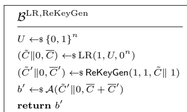
Fig. 7. Adversary \mathcal{B} for UP-IND using as a subroutine the adversary \mathcal{A} attacking 1-circular security of EncBad.
