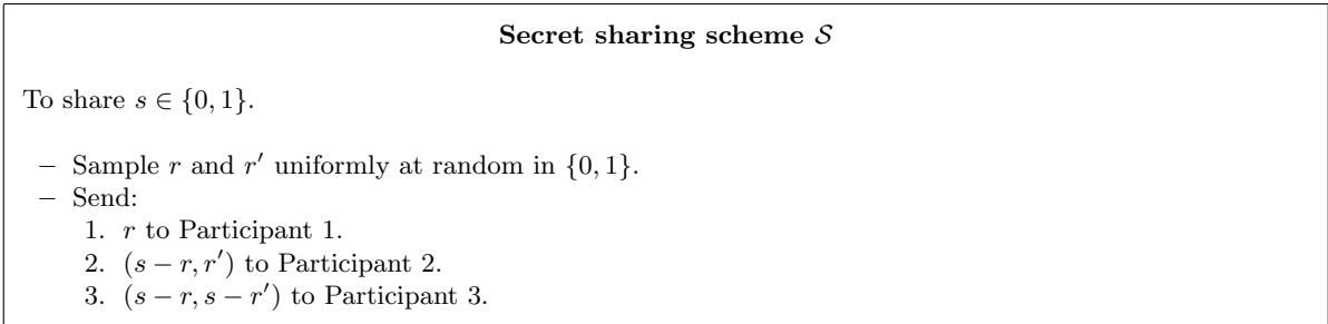
Fig. 5. A 2-out-of-3 threshold linear secret sharing scheme \mathcal{S}
