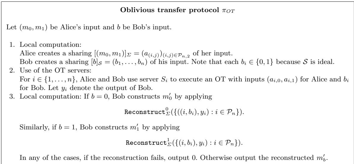
Fig. 3. Protocol \pi_{OT} for ideal LSSSs.
