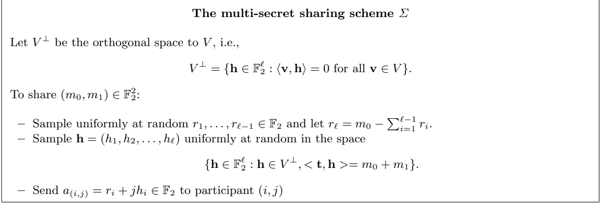
Fig. 2. The multi-secret sharing scheme \Sigma
