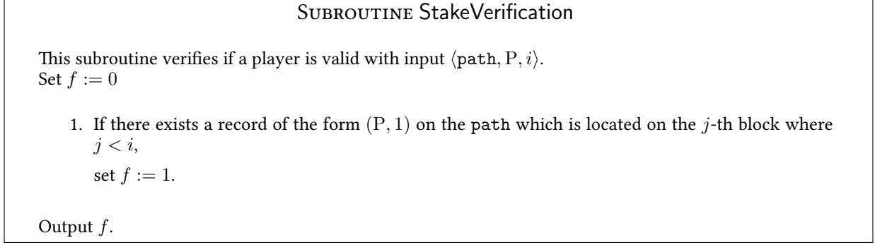
Figure 11: Stake verification subroutine StakeVerification.
