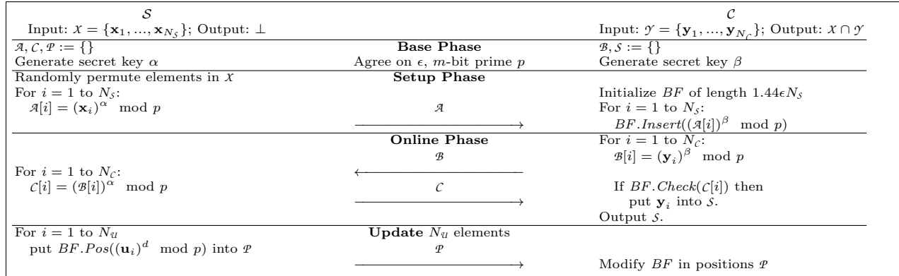
Fig. 2: The Diffie-Hellman-based PSI protocol (DH-PSI).
