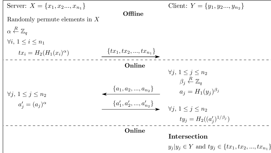
Fig. 1. Basic PSI protocol proposed in [5] that relaxes the security of the [25] to be secure against semi-honest adversaries. H_1 and H_2 are hash functions modeled as random oracles. [5, Adapted].
