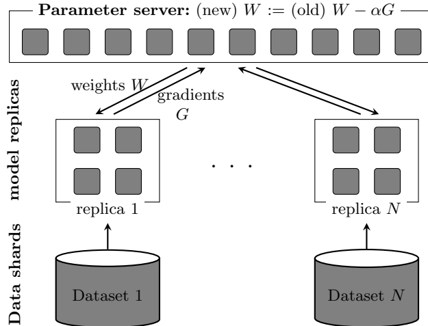
Fig. 2. Asynchronous SGD [11, 21].
