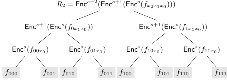
Fig. 2. Using Lipmaa’s (w, 1) -CPIR from [Lip05] with w = 2 and n = 8 . The receiver sends \text{Enc}^s(x_0) , \text{Enc}^{s+1}(x_1) , \text{Enc}^{s+2}(x_2) to the sender. The sender computes recursively the values at intermediate nodes, and then replies with R_2 .
