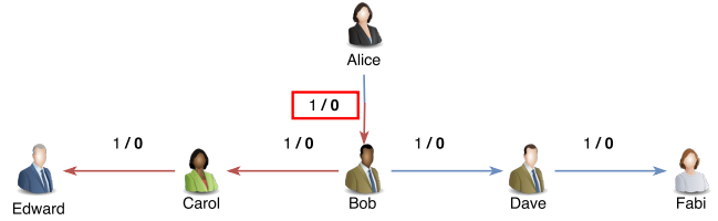
Figure 10: Execution depicting two payments: payment \text{Txid}_i from Alice to Edward and payment \text{Txid}_j from Alice to Fabi. If Alice and Bob are byzantine, they can allow both payments to be successful (while losing funds themselves).
