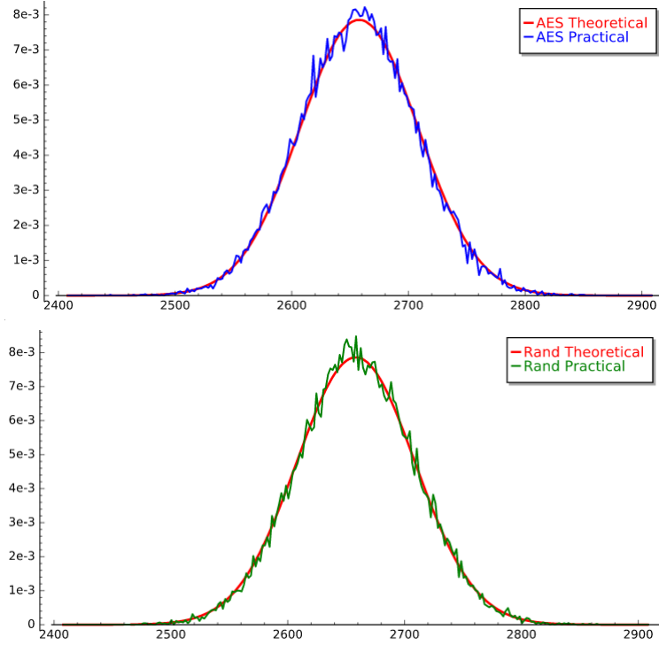
Figure 3: Probabilistic Distributions of the Number of Sets \mathcal{S} that satisfy the required property for 5-round AES and for a Random permutation - using 20 000 initial cosets.
