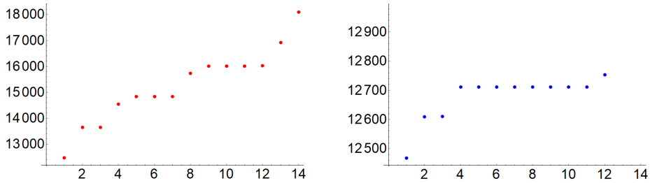
Figure 1: Natural logarithms of lengths of lattice basis vectors in the Boneh-Durfee .284 attack with n \approx 2^{6,000} and \delta \approx .284 , before and after lattice basis reduction.
