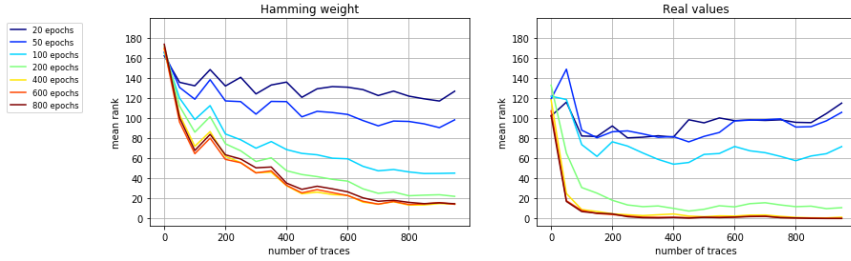
Figure 14: Mean ranks of \text{MLP}_{\text{best}} with Hamming weights as labels and \text{MLP}_{\text{best}} with real values as labels.
