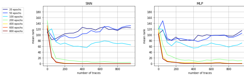
Figure 13: Mean ranks and accuracy of a SNN and a MLP with different numbers of epochs.
