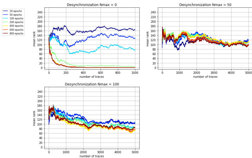
Figure 33: Mean ranks of MLP best for a desynchronization amount in \{0, 50, 100\} and different values of epochs.
