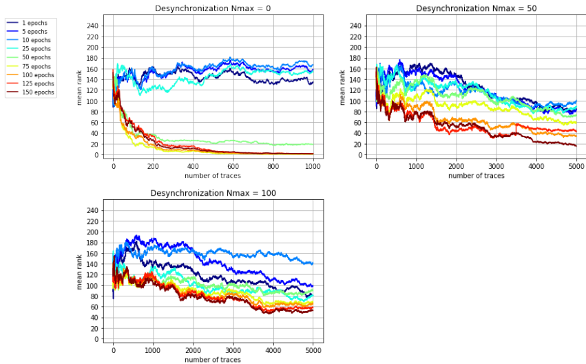
Figure 31: VGG-16 mean ranks for a desynchronization amount in \{0, 50, 100\} and different numbers of epochs.
