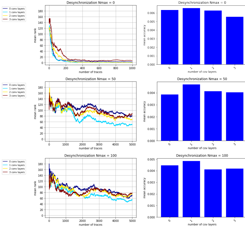
Figure 24: For a desynchronization amount in \{0, 50, 100\} and different numbers of CONV layers per block, the mean ranks (left-hand side) and the mean accuracy (right-hand side) of \text{CNN}_{\text{base}} .
