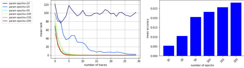
Figure 16: Mean ranks and accuracy of \text{MLP}_{\text{best}} on a first order SCA.
