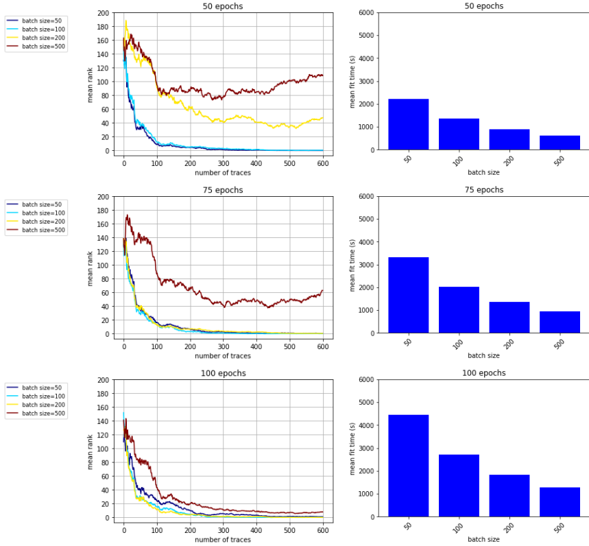
Figure 21: Mean ranks and training time of \text{CNN}_{\text{base}} with different values of epochs and batch sizes.
