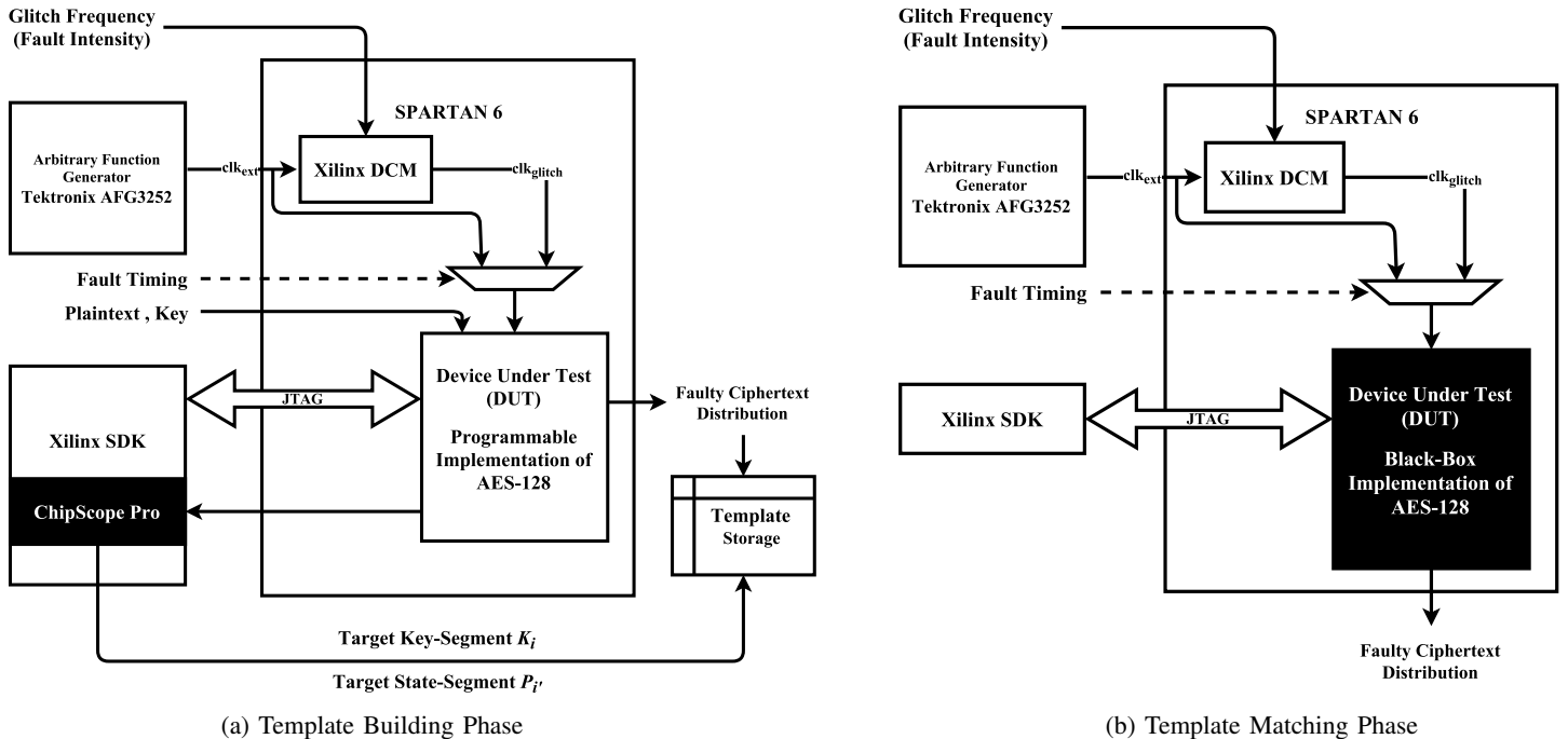
Fig. 2: Experimental Set-Up
