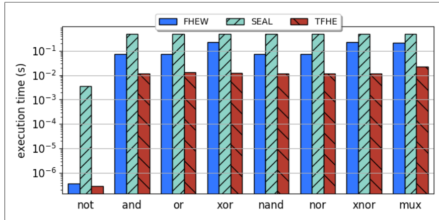
Fig. 7. Gate speed for FHEW, SEAL, and TFHE.
