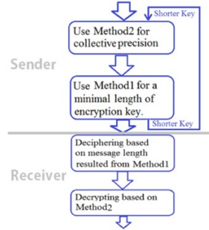
Figure 4. Sender and Receiver
