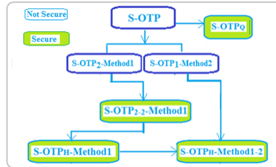
Figure 7. The road to information conservational security
