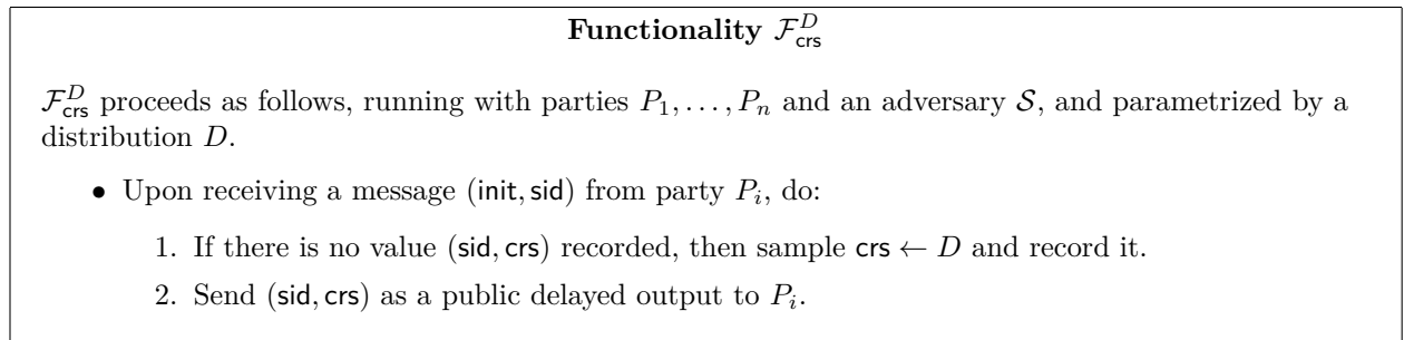
Figure 9: The common reference string functionality
