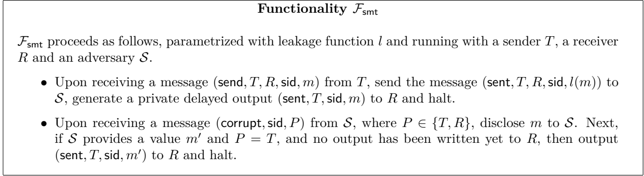
Figure 10: The secure message transmission functionality
