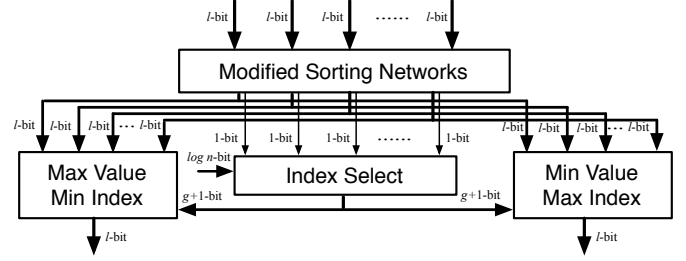
Fig. 5. The complete circuit design for M - g - U . n is the number of sensors, l is the length of the endpoint of the input interval, and g is the number of faulty sensors.
