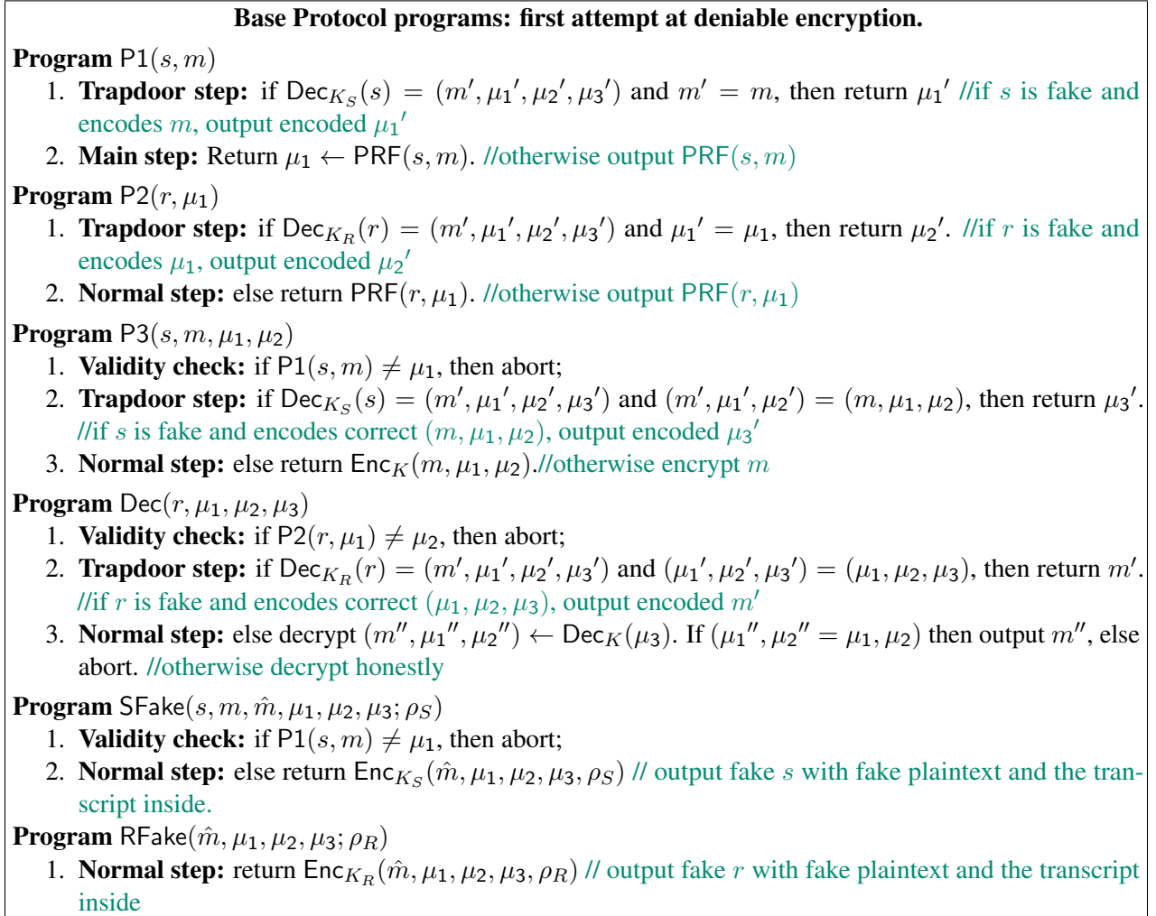
Figure 3: Base Protocol programs: first attempt at deniable encryption. P1, P2, P3, Dec are deterministic; 14 SFake, RFake are randomized.
