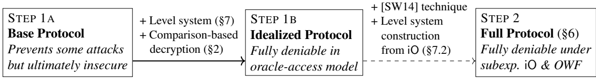
Figure 1: The construction, step by step. The second arrow is dashed because while conceptually the Idealized Protocol is a stepping-stone to the Full Protocol, technically the Full Protocol requires very different techniques, and must be proven from scratch rather than “building on” the Idealized Protocol.
