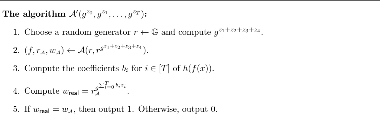
Figure 1: The adversary \mathcal{A}' that breaks the entropic power-DDH assumption.
