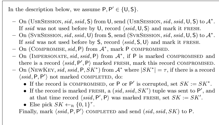
Fig. 7: Adaptively Secure Functionality \mathcal{F}_{\text{AKE-KCI}}
