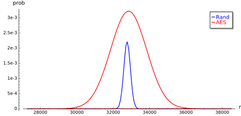
Fig. 2. Comparison between the theoretical probabilistic distribution of the number of collisions between small-scale AES and a random permutation.
