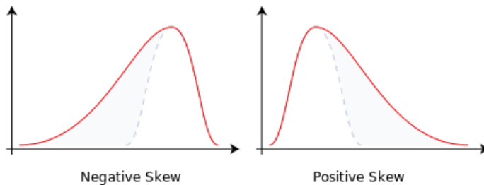
Fig. 4. Examples of negative and positive skew.
