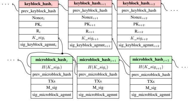
Figure 1: A figure presentation of the blockchain structure. This example contains three pinned keyblocks ( i, i + 1 , and i + 2 ), and three pinned microblocks ( j, j + 1 and j + 2 ). Microblock j and j + 1 were created by the leader determined by keyblock i , and microblock j + 2 was created by the leader determined by keyblock i + 1 .
