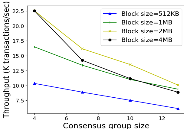
Figure 3: Throughput of RepuCoin.
