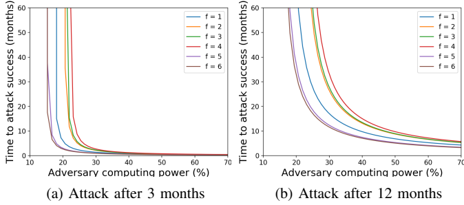
Figure 4: Minimum effort to break the liveness of RepuCoin. We consider cases where an attacker joins after the system has operated for 3 months and a year, and where the consensus group controls mining power ranging from 44.7% (i.e., f=1, |\mathbb{X}| = 4 ) to 98.1% (i.e., f=6, |\mathbb{X}| = 19 ). The x-axis shows the needed computing power and the y-axis shows the required time to attack the system.
