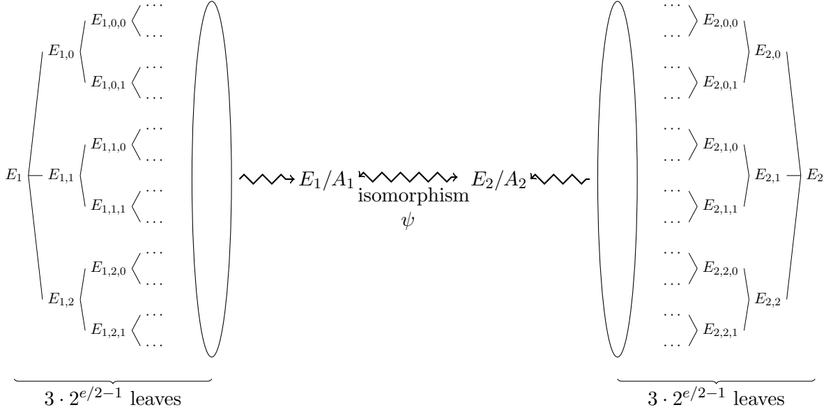
FIGURE 1. Meet-in-the-middle attack for degree-2 isogeny trees.
