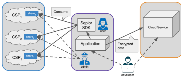
Fig. 7. Sepior High Level Architecture
