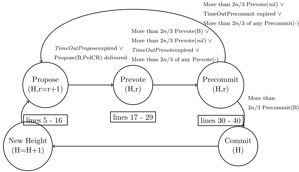
Figure 1: State Machine for Tendermint One-Shot algorithm described in Figure 3. For ease of readability, common exit conditions are represented.
