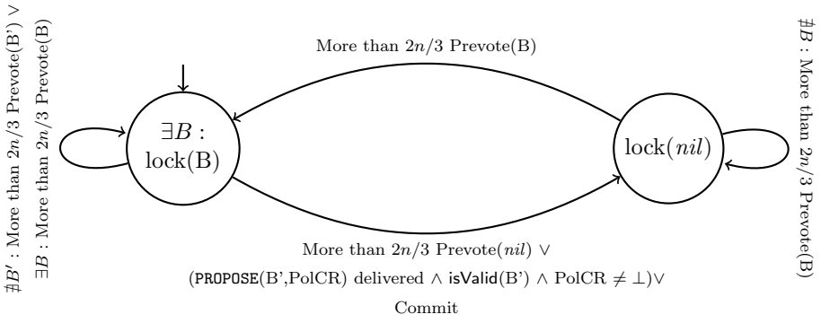
Figure 2: State machine Lock/Unlock
