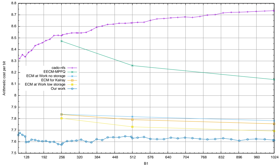
Fig. 1. Arithmetic cost per bit for the scalar multiplication of ECM stage 1 of ECM assuming S = 1M .
