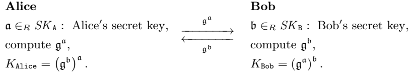
Fig. 2. Outline of SIDH Protocol (Crypto-friendly Description).
