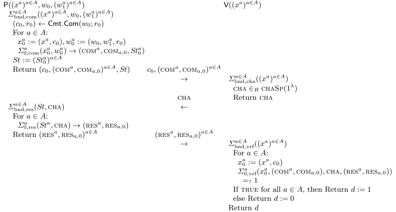
Fig. 1. The protocol \Sigma_{\text{bnd}}^{a \in A} of our proof system \Pi_{\text{bnd}}^{a \in A} for the NP witness relation R_{\text{bnd}}^{a \in A} .
