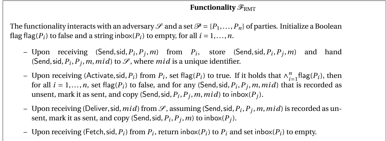
Figure 3: The reliable message transmission ideal functionality in the synchronous setting.
