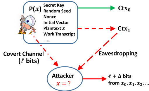
Fig. 1. Setting of Steal-Entropy and Steal Resilient Encryption. A Trojan horse malware can observe all (secret) information during the execution of algorithm P(\cdot) , including input x = x_0 \| x_1 \| x_2 \| \dots ( x_i \in \{0, 1\} ), secret keys, random seeds, IV values, ciphertext ( Ctx_0 \| Ctx_1 ), and all step-by-step work transcript, but is only able to deliver at most \ell (here we assume \ell < |x| ) bits message to the remote attacker via some unidirectional covert channel. With these \ell bits stolen-message and whatever he could eavesdrop over Internet, the remote attacker attempts to output \ell + \Delta bits values among x_i 's. This paper proposes to “encode” the output of P as two parts: a smaller part Ctx_0 ( |Ctx_0| > \ell + \lambda where \lambda is the security parameter) and a large part Ctx_1 , and transfer or store the small part Ctx_0 using more secure manner, such that the adversary has to resort to advanced technique to steal information about Ctx_0 (e.g. using the Trojan horse virus and the covert channel), rather than eavesdropping. We remark that, (1) we are only interested in length-preserving encryption, such that the bit length of ciphertext (i.e. |Ctx_0| + |Ctx_1| ) is equal to the bit length of plaintext; (2) since |Ctx_0| > \ell + \lambda , so that the attacker could not steal full knowledge of Ctx_0 via the covert channel; (3) typically, \ell \geq \text{SECRETKEYSIZE} , so the Trojan horse malware may steal the entire secret key. For example, \ell = 10000 and \text{SECRETKEYSIZE} = 128 or 256 for AES, or \text{SECRETKEYSIZE} \leq 4096 for typical RSA private key.
