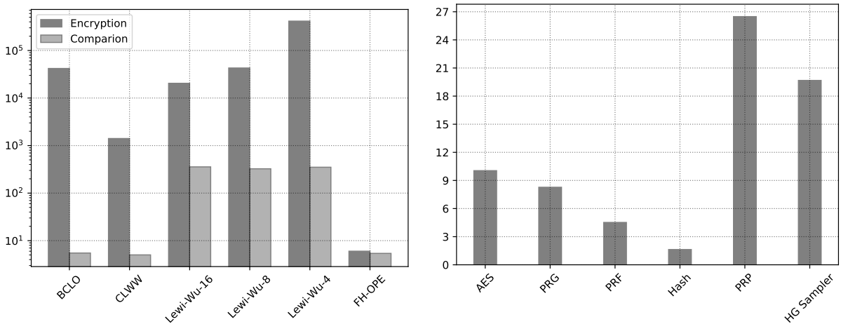
(a) Schemes benchmark (time in microseconds, log scale). Lewi-Wu parameter is the number of blocks.
