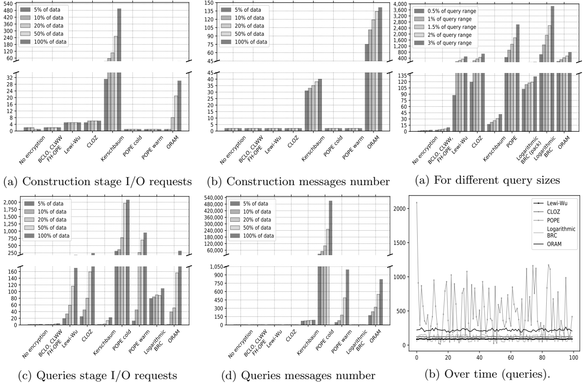
Figure 3: Protocol scalability
