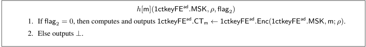
Figure 7: This circuit h is an input of the key generation algorithm of 1\text{keyFE}^{\text{sk}} (selectively secure, single-key, and succinct secret-key FE). This circuit outputs an encryption of m under the master secret key of 1\text{ctkeyFE}^{\text{ad}} .
