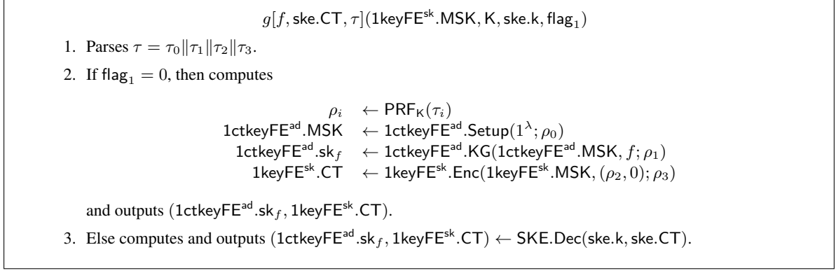
Figure 6: This circuit g is an input of the key generation algorithm of \text{ssFE}^{\text{pk}} (selectively secure and succinct public-key FE). This circuit outputs a functional decryption key of f by the single-key and single-ciphertext scheme and an encryption of randomness that will be used in the circuit h under the master-key of the single-key scheme.
