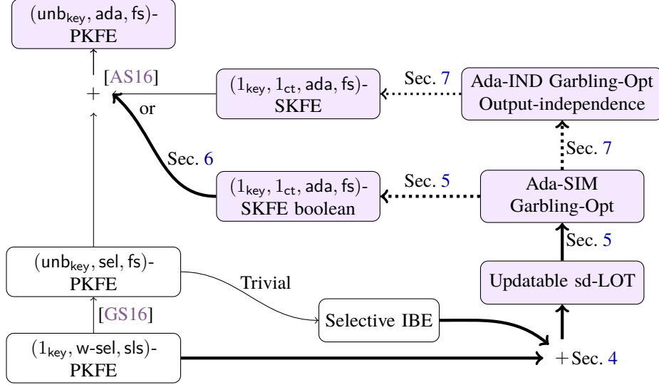
Figure 1: Illustration of the path from our starting point to the goal: In this figure, “SKFE boolean” denotes SKFE for boolean circuits. “Updatable sd-LOT” denotes selective-database updatable laconic OT. Regarding garbling scheme, “Garbling-Opt” denotes garbling schemes with nearly optimal online complexity and “Output-independence” denotes the online complexity does not depends on output-length (See Sections 5 and 7 for more details). Ada-SIM/Ada-IND denote simulation-/indistinguishability-based adaptively secure garbling schemes, respectively. Solid thin arrows denote known or trivial implications. Thick solid and dotted arrows denote implications that we prove in this study. Here, in the case of dotted lines, we assume specific properties of underlying tools. See each section for details.
