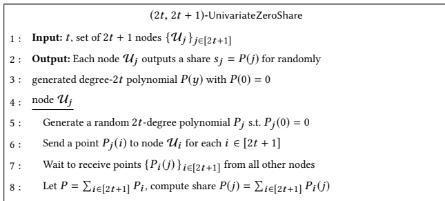
Fig. 9. (2t, 2t + 1) -UnivariateZeroShare between 2t + 1 nodes. A 0-hole univariate polynomial P of degree- 2t is generated.
