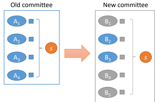
Fig. 1. Handoff between two committees at the end of a dynamic proactive secret-sharing epoch. The secret s remains fixed. Committees may intersect, e.g., B_2 = A_2 and B_3 = A_3 .
