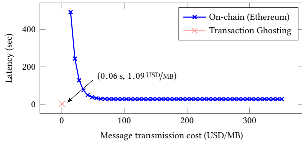
Fig. 7. Tradeoff in latency vs. message transmission cost. The blue curve shows the on-chain tradeoff. The red dot at (0.06 s, 1.09 USD/MB) corresponds to Transaction Ghosting.
