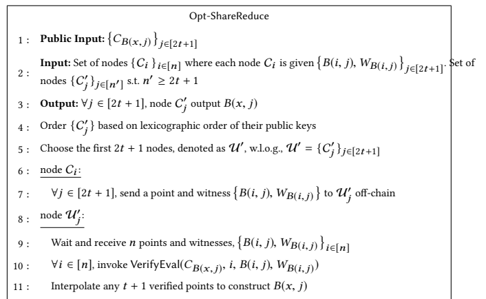
Fig. 11. Opt-ShareReduce between the committees C and C' .
