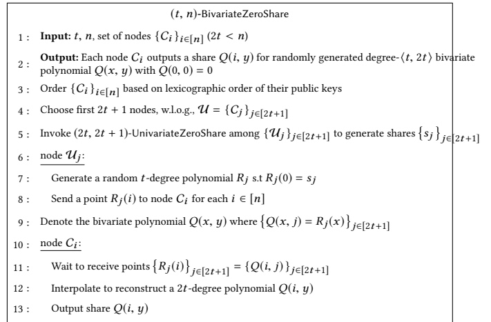
Fig. 10. (t, n) -BivariateZeroShare between n nodes. A 0-hole bivariate polynomial Q of degree- \langle t, 2t \rangle is generated.
