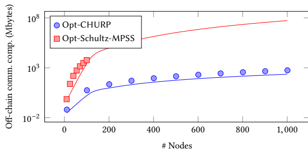
Fig. 6. Concrete off-chain communication complexity for Opt-CHURP and Schultz-MPSS, with log-scale y-axis. Points show experimental results; expected polynomial curves (respectively quadratic and quartic) are also shown.
