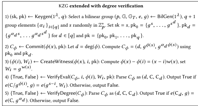
Fig. 18. KZG [45] extended with degree verification.
