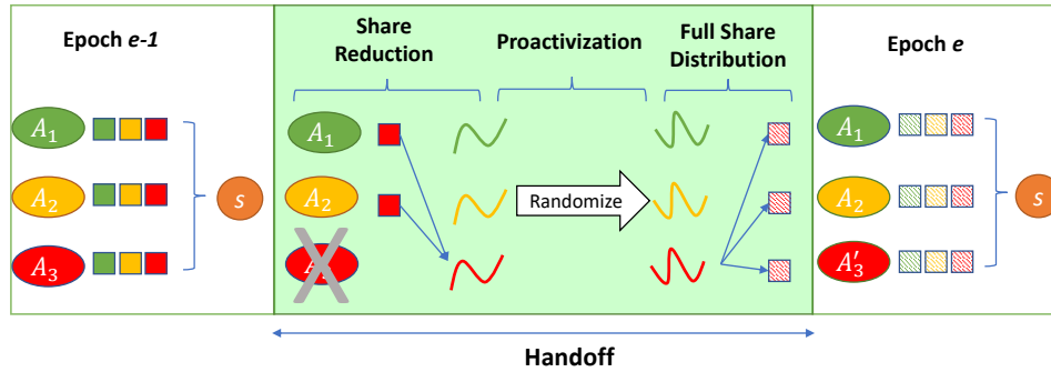
Fig. 3. An example of the handoff protocol: Curves denote univariate polynomials (reduced shares) while squares denote points on these polynomials. See Section 3.3 for a description.
