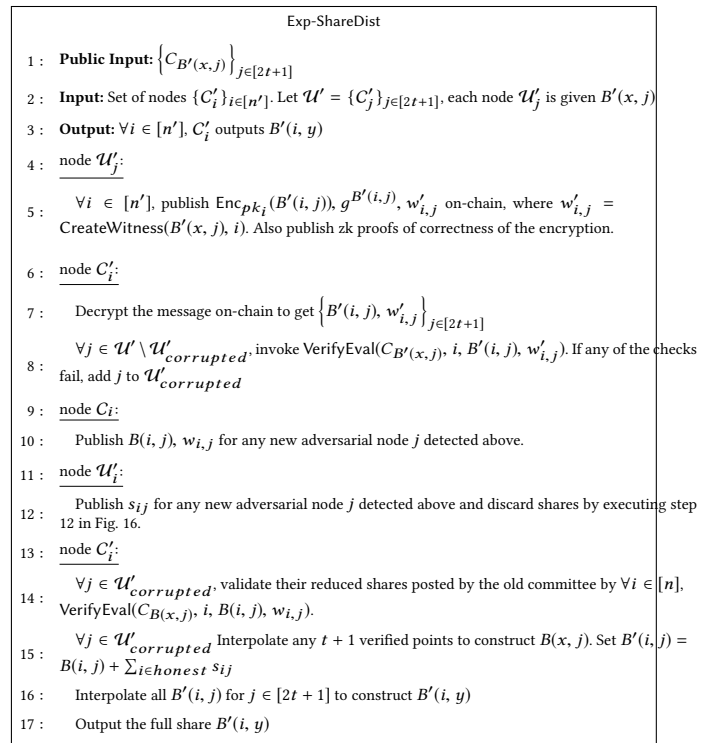
Fig. 17. Exp-ShareDist protocol.
