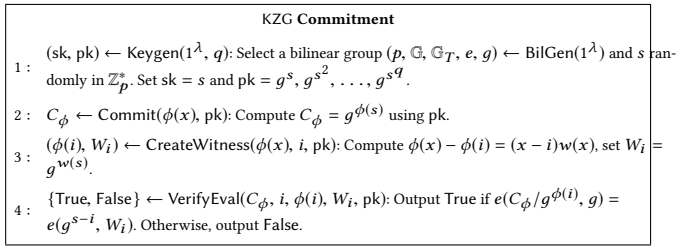
Fig. 8. Protocols of KZG commitment scheme.
