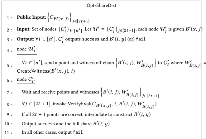
Figure 13: Opt-ShareDist uses the updated reduced shares to distribute full shares in C' .
