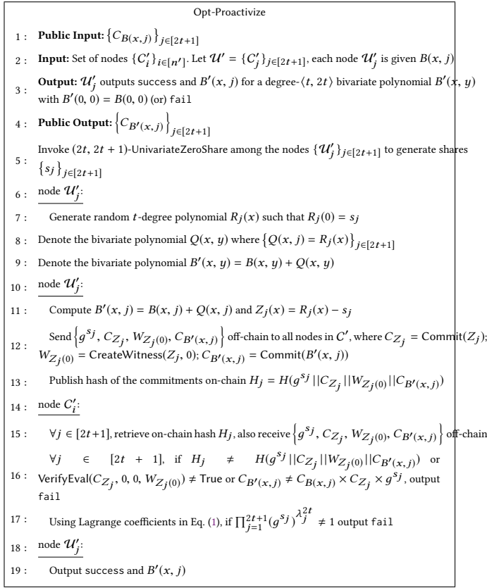
Figure 12: Opt-Proactivize updates the reduced shares.
