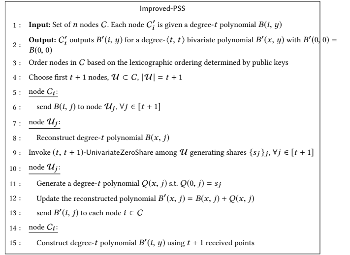
Figure 14: Improved PSS for static setting, honest-but-curious adversary.
