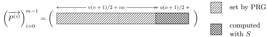
Fig. 1. Petzoldt's compression technique.
