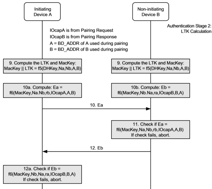
Fig. 4. Phase 4 – Session Key Derivation and Validation
