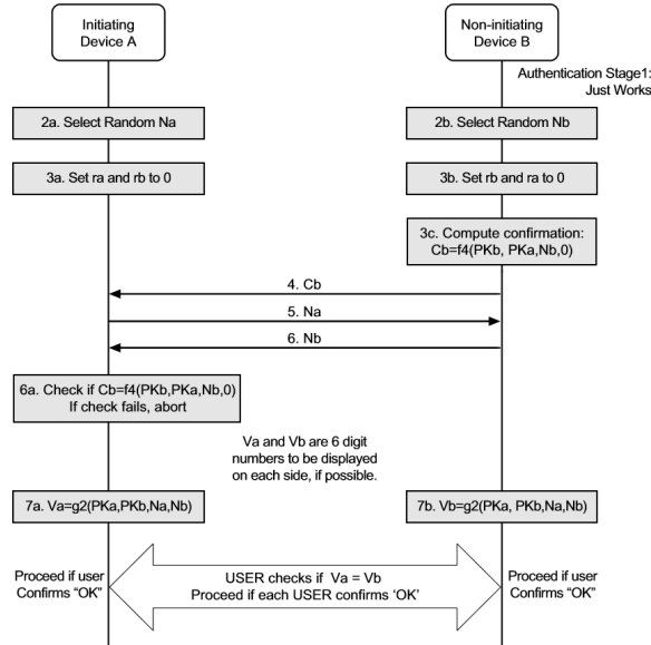
Fig. 2. Phase 3 – Authentication (Numeric Comparison)
