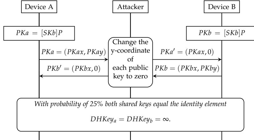
Fig. 6. Fixed Coordinate Invalid Curve Attack – Phase 2
