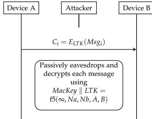
Fig. 7. Semi-Passive MitM Attack – Passive Eavesdropping
