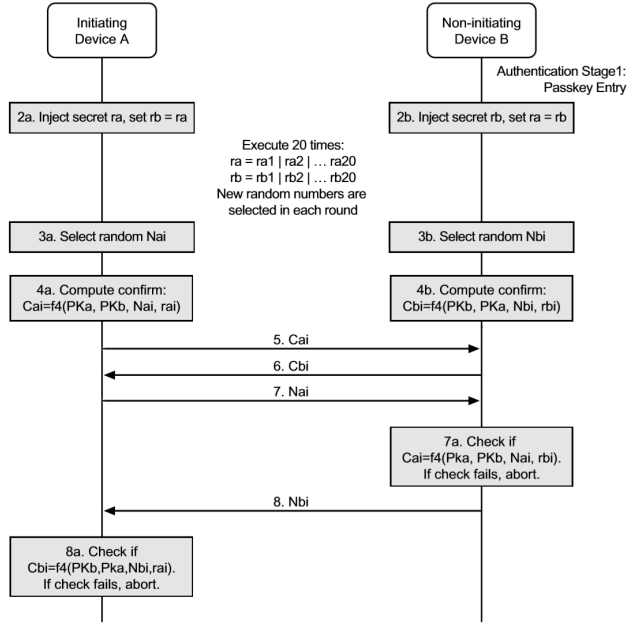
Fig. 3. Phase 3 – Authentication (Passkey Entry)
