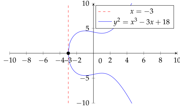
Fig. 5. Example of an elliptic curve with an order-two point at (-3, 0)
