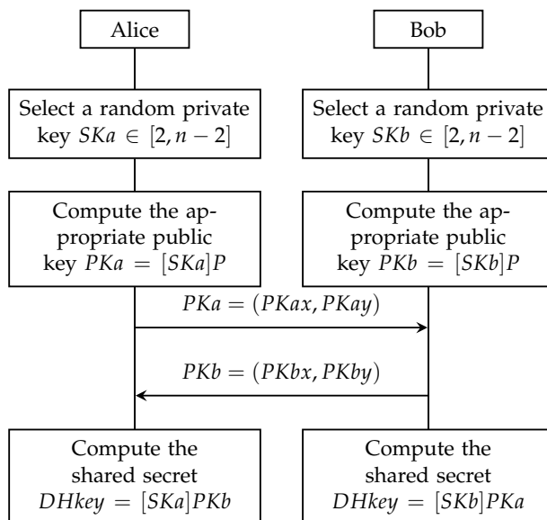
Fig. 1. Elliptic Curve Diffie-Hellman Protocol Diagram
