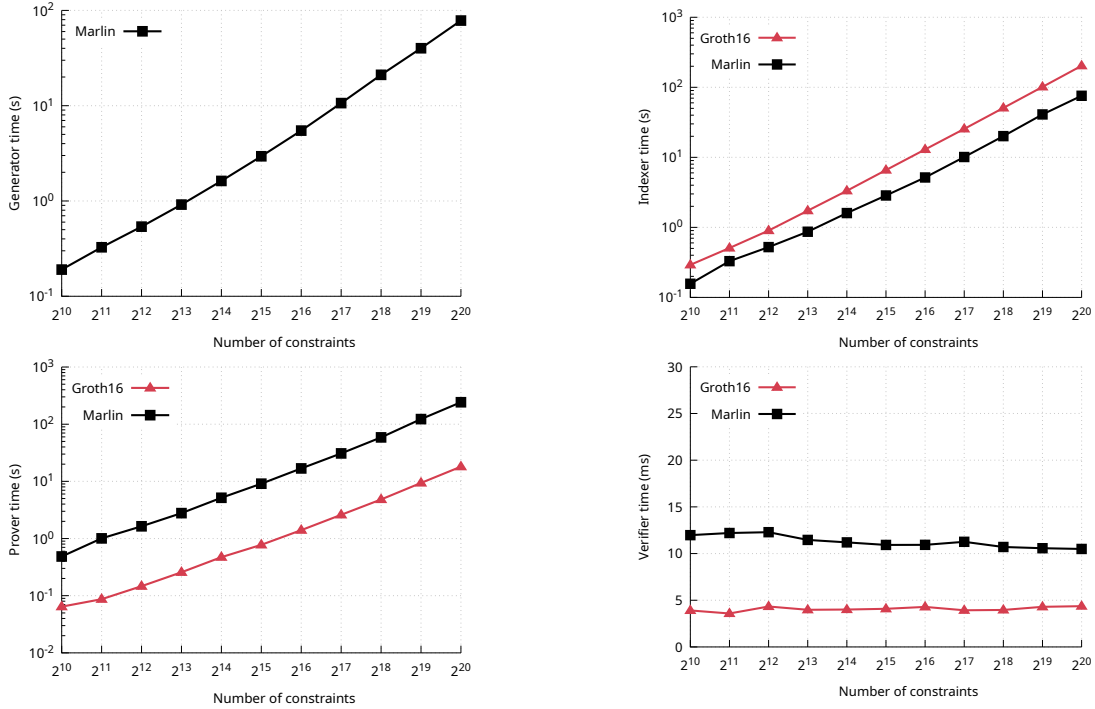
Figure 2: Measured performance of MARLIN and [Gro16]. We could not include measurements for [MBKM19, Sonic] because at the time of writing there is no working implementation of its unhelped variant.
