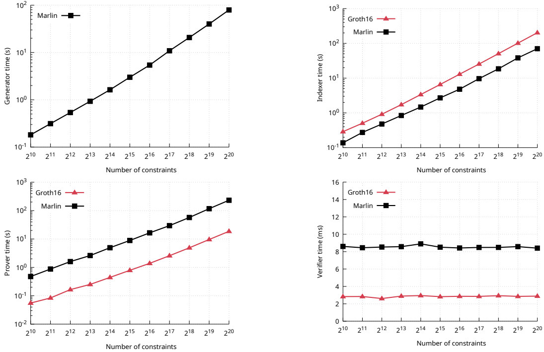
Figure 2: Measured performance of MARLIN and [Gro16]. We could not include measurements for [Mal+19, Sonic] because at the time of writing there is no working implementation of its unhelped variant.
