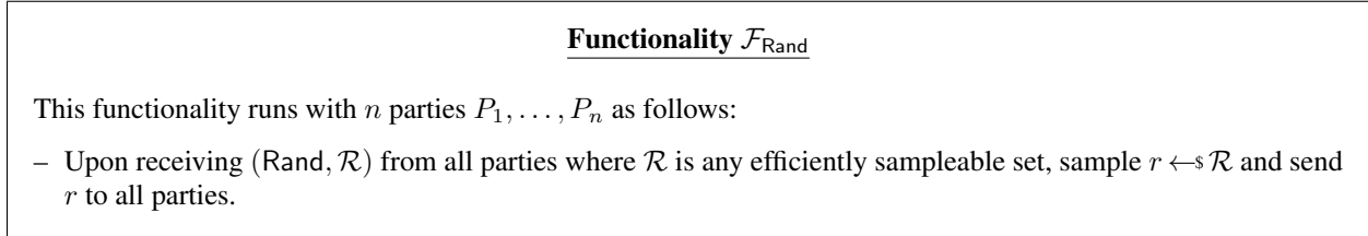
Figure 11: Coin-tossing functionality.
