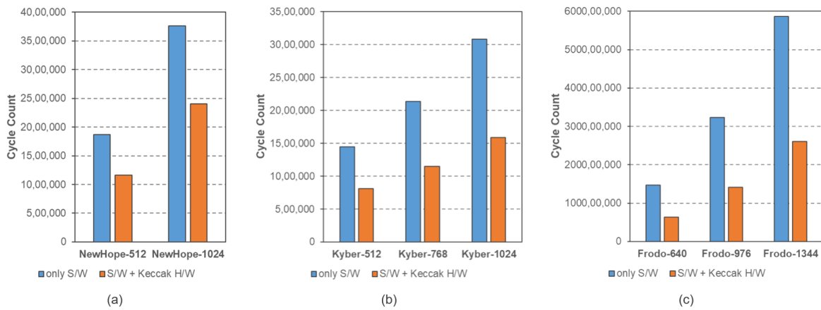
Figure 25: Comparison of cycle counts of (a) NewHope, (b) CRYSTALS-Kyber and (c) Frodo CCA-KEM-Encaps with and without hardware-accelerated Keccak.
