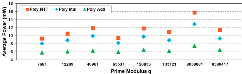
Figure 29: Power consumption of polynomial arithmetic operations for different prime moduli.
