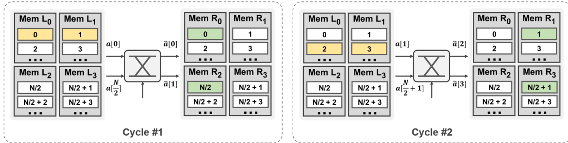
Figure 6: Data-flow of our NTT memory architecture in the first two cycles (butterfly inputs are in yellow and outputs are in green).
