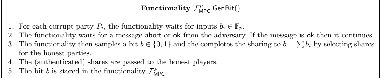
Figure 5. The ideal functionality for single random bits
