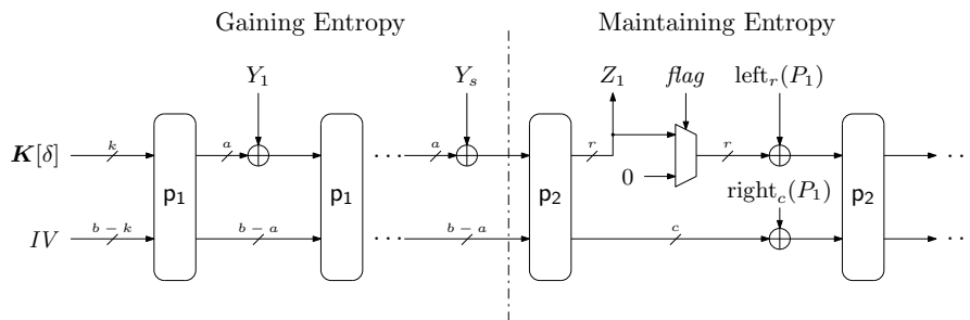
Fig. 3: The duplex construction as used by Taha and Schaumont [38] and ISAP [17].
