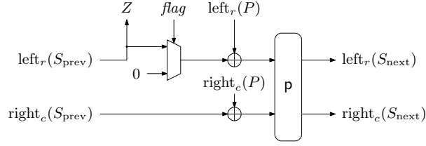
Fig. 2: An evaluation of \text{KD.duplex} , with its previous state S_{\text{prev}} and next state S_{\text{next}} are indicated. Intuitively, leakage occurs on both states, and the leakage function \mathbf{L} returns \lambda bits of leakage.
