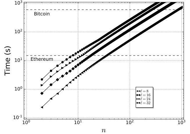
Figure 1: Maximum round computation time
