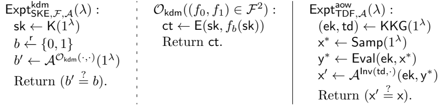
Figure 2: The KDM security experiment for an SKE (left), the KDM-encryption oracle used in the KDM security experiment (center), and the adaptive one-wayness experiment for a TDF (right).
